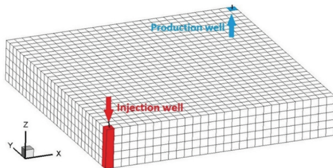
Figure 1: Calculation domain and well locations
