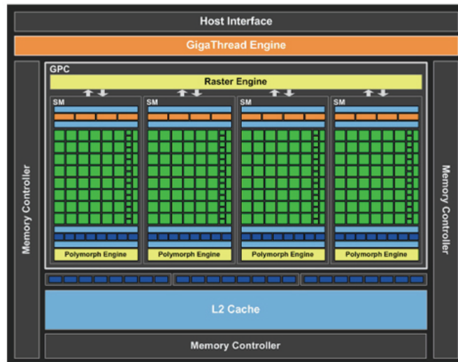
Figure 12: Fermi Architecture for NVIDIA GeForce GTX550Ti
