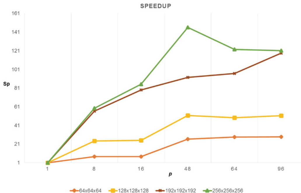
Figure 10: Change of speedup S_p values depending on N_x \times N_y \times N_z and p
