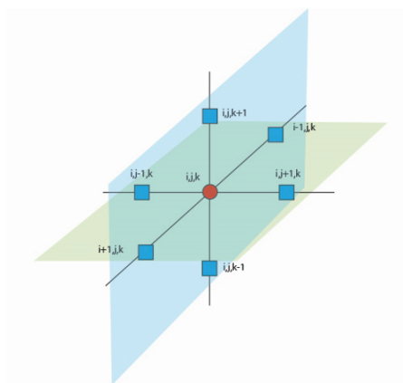
Figure 2: Numerical scheme of Jacobi method
