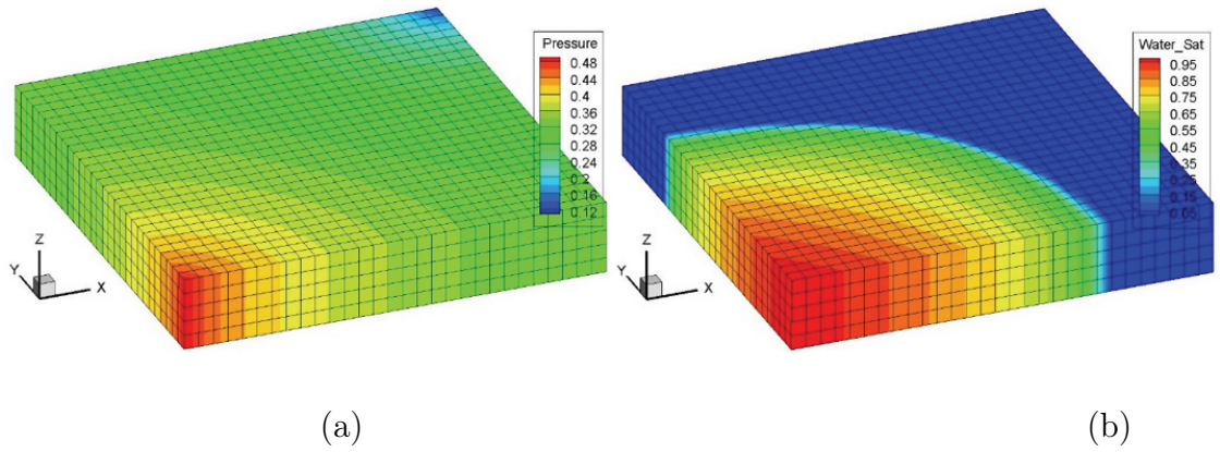
Figure 3: Distribution of (a) pressure and (b) water saturation
