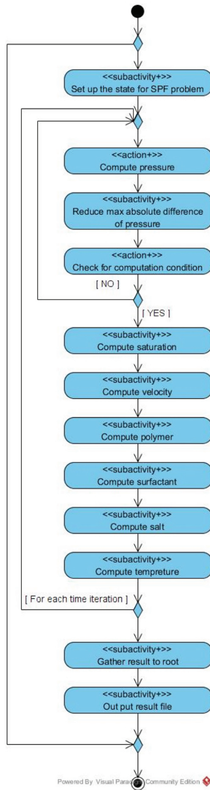
Figure 9: Activity diagram of parallel computation of SPF problem in each processing element
